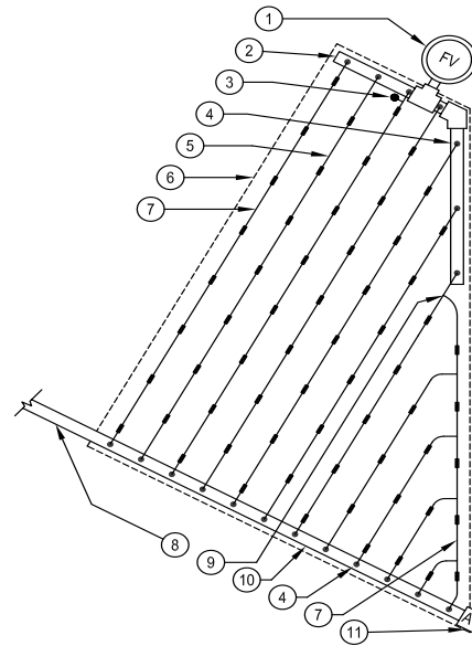
Detail No.20 Island Layout End Feed
