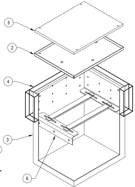
CORNER ELEVATION:
